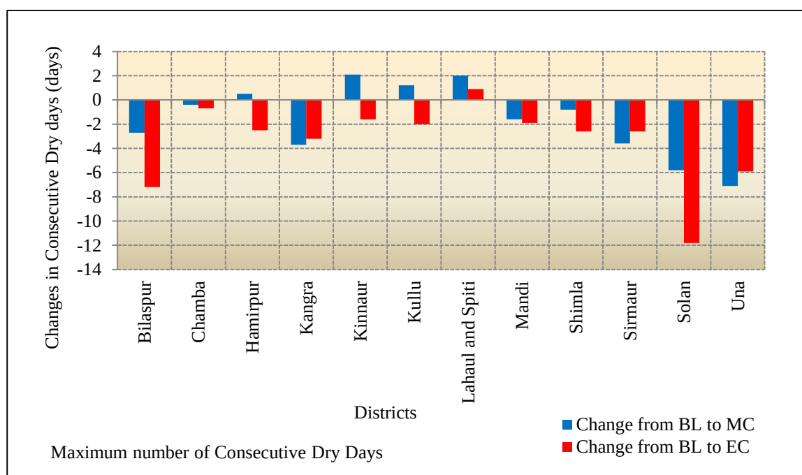
Figure 32 : Characteristics of Precipitation Extremes - consecutive Dry and Wet days
