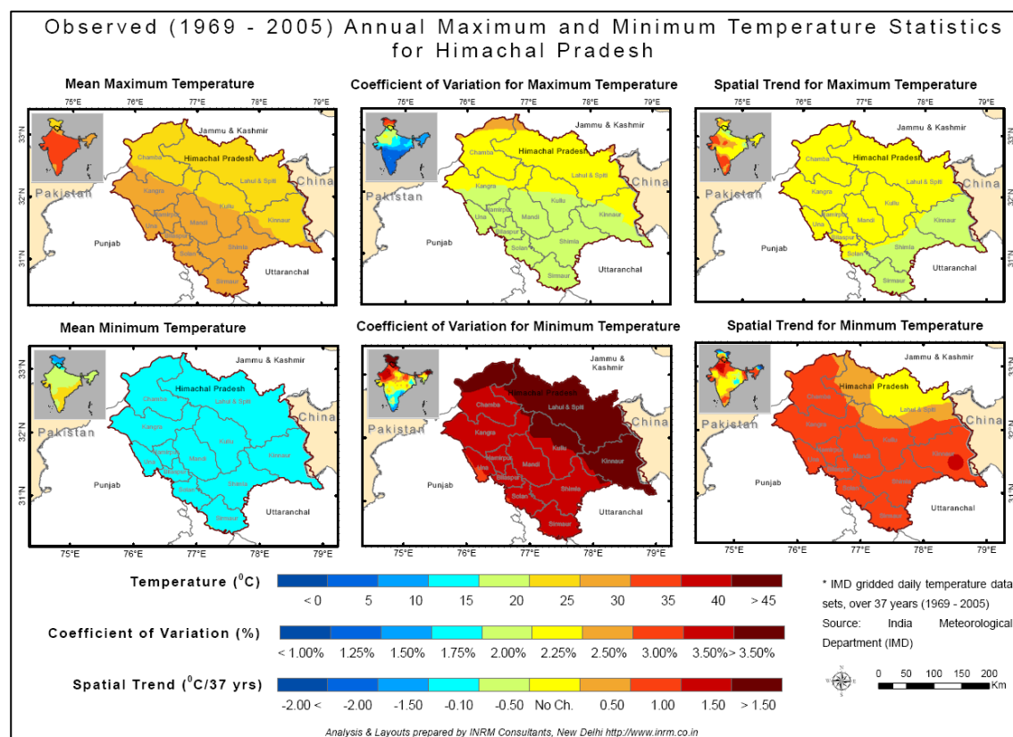
Figure 10 : Observed annual maximum and minimum temperature statistics in Himachal Pradesh
