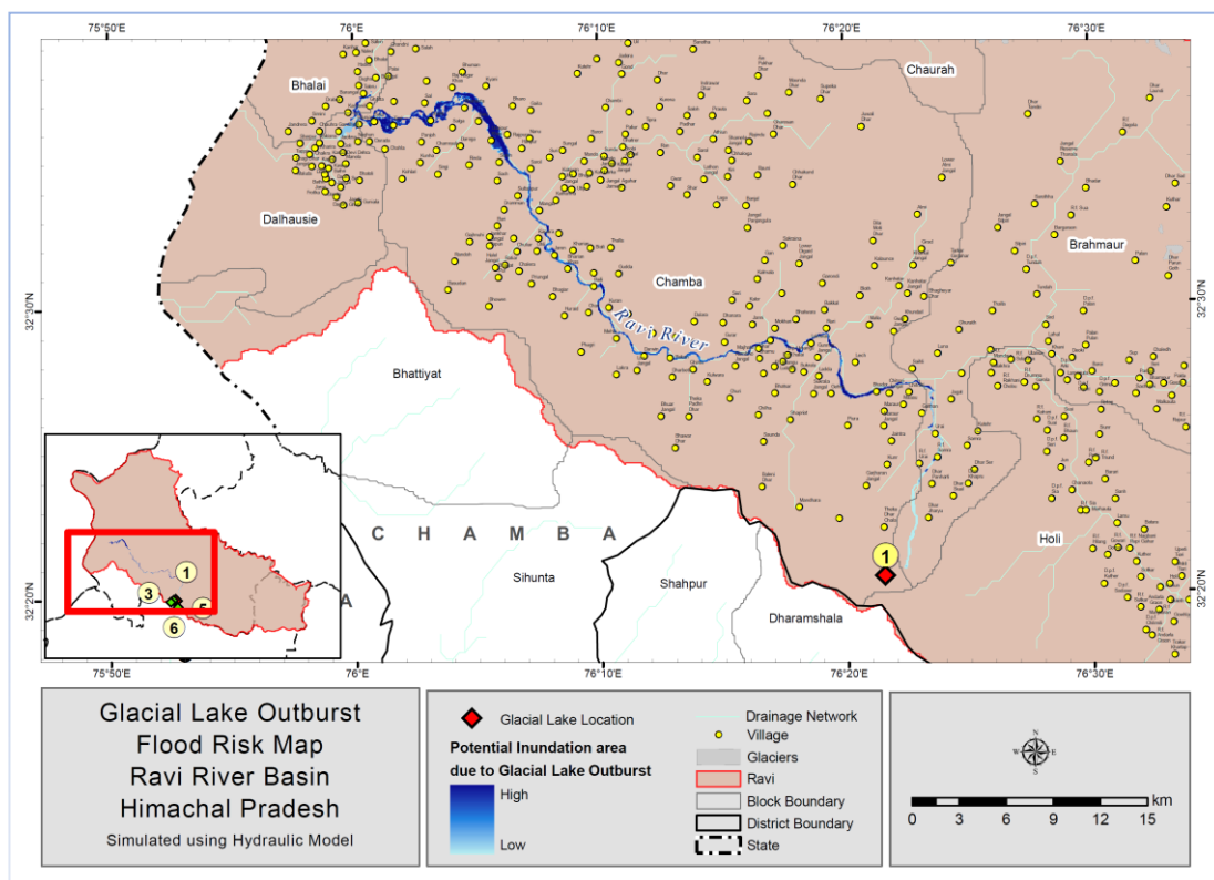
Figure 39 : Simulated Inundation caused due to Glacial Lake Outburst Flood in Ravi basin (Himachal Pradesh)
