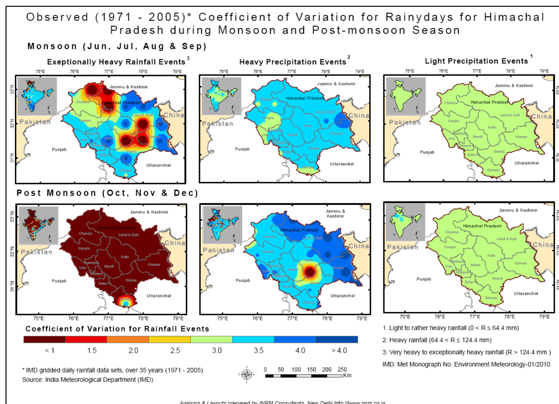
Figure 8 : Observed rainfall Statistics – Inter annual variation in rainy days during Monsoon and Post-monsoon season
