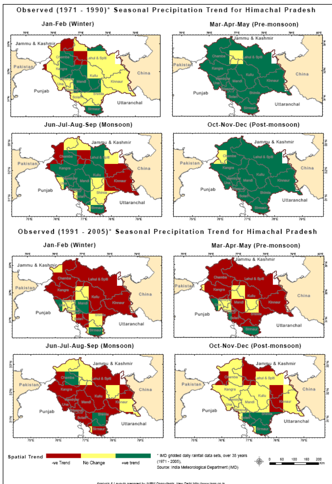
Figure 6 : Observed seasonal rainfall trends in Himachal Pradesh (1971-1990 and 1991-2005)
