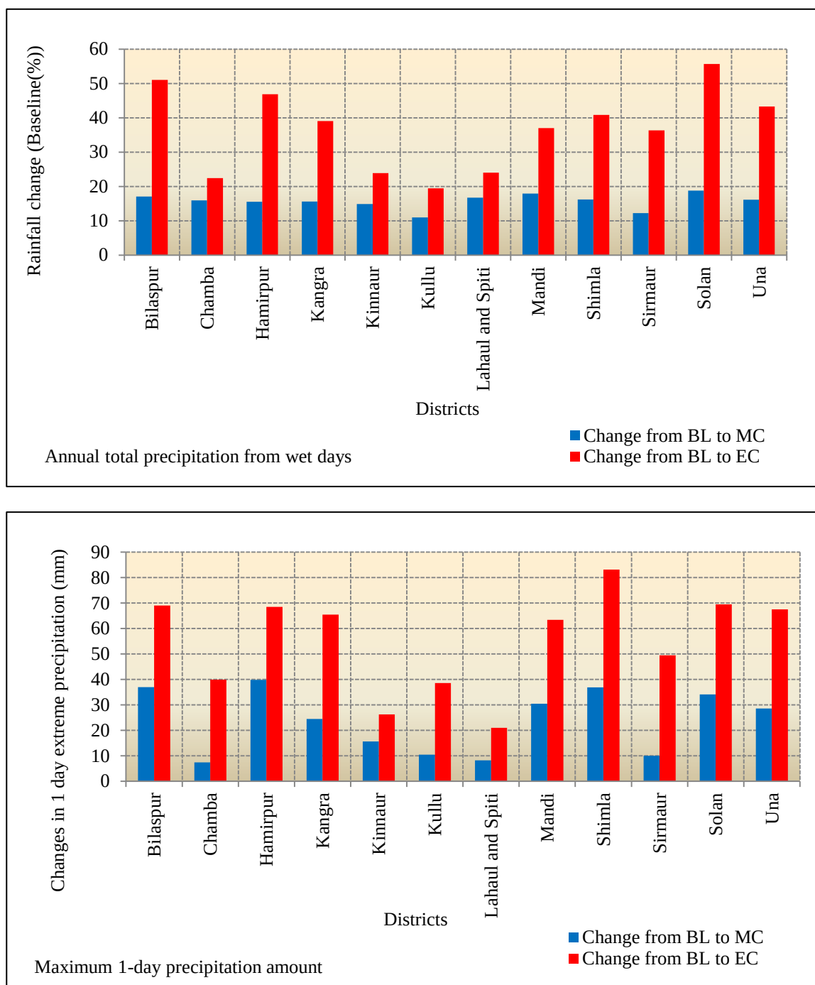
Figure 33 : Characteristics of Annual Precipitation, Maximum 1 day and Maximum 5 day precipitation and Simple Daily Intensity Index
