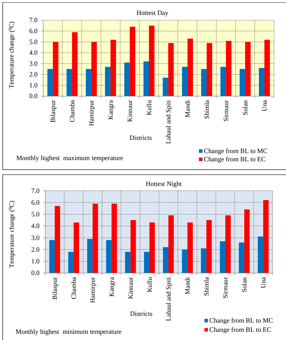
Figure 28 : Characteristics of Hottest day and Hottest night, Coolest day and Coolest night
